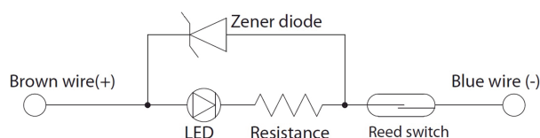
[ Sensor Circuit Diagram ]
